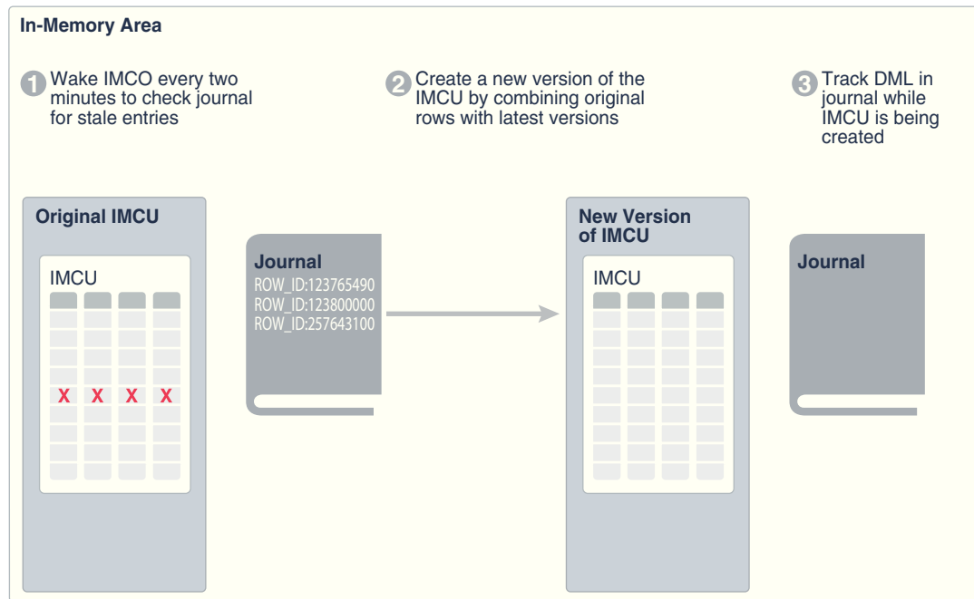
Figure 9-4 Trickle Repopulation
