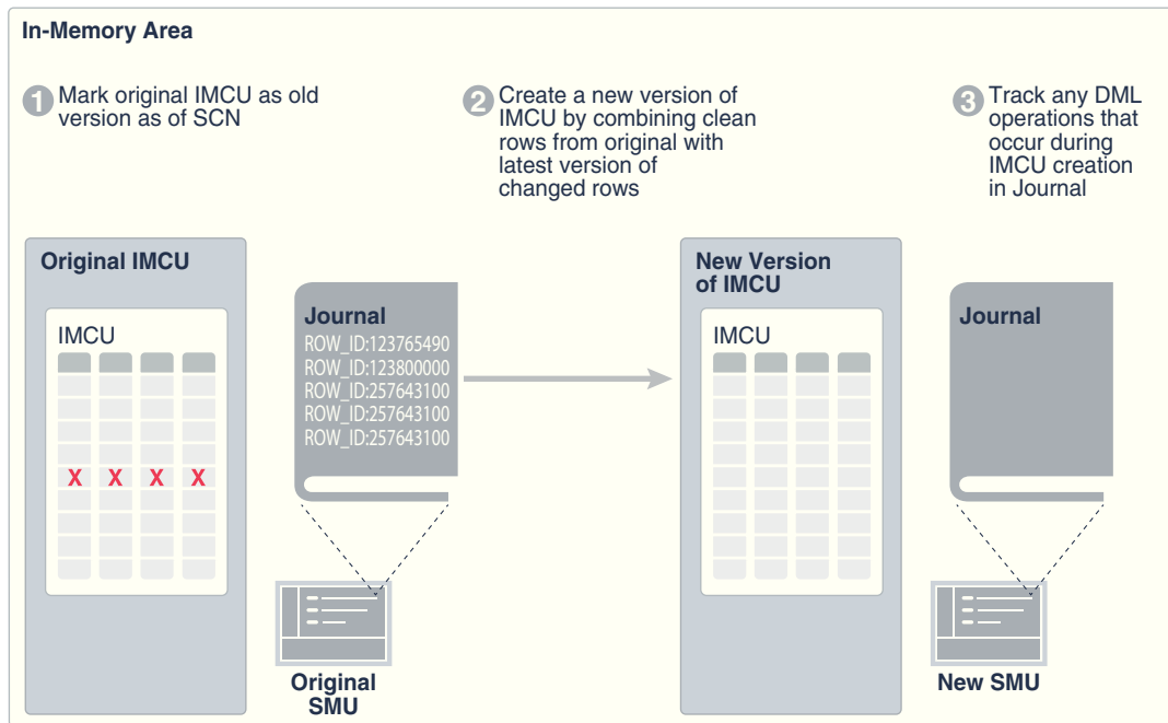
Figure 9-1 Double Buffering
