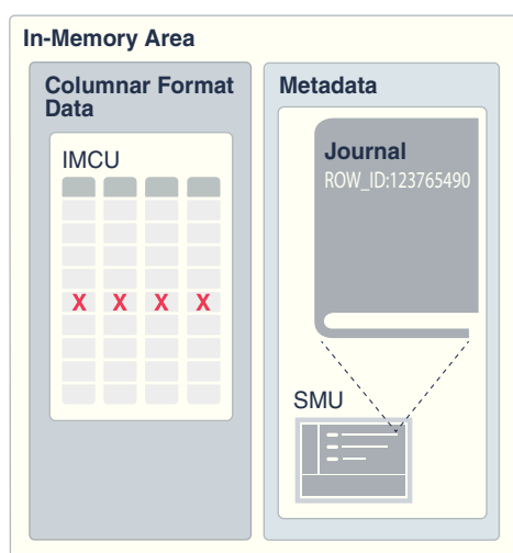
Figure 2-11 Transaction Journal
