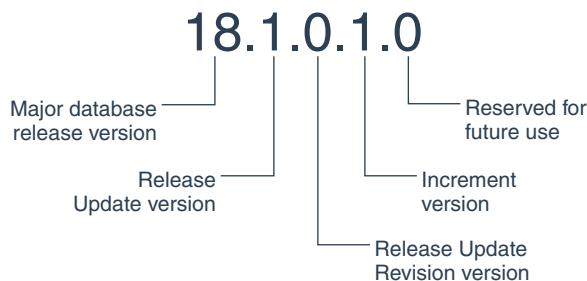
Figure 1-2 Example of an Oracle Database Release Number
