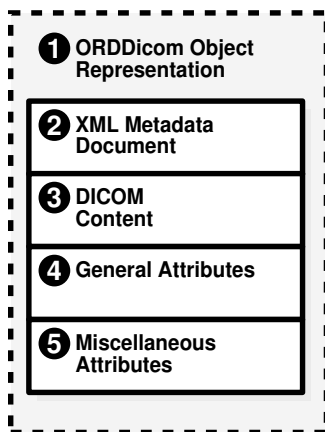
Figure 2-2 ORDDicom Object
