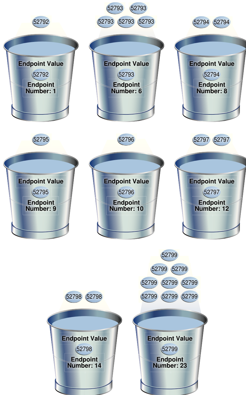
Figure 11-2 Frequency Histogram
