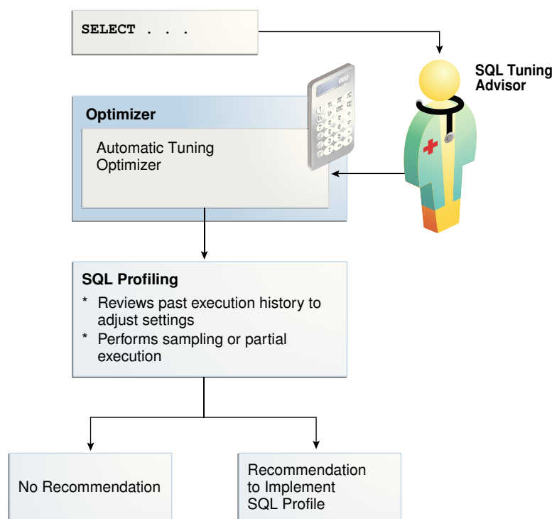
Figure 25-5 SQL Profiling
