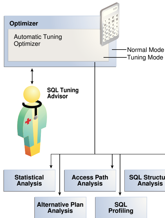
Figure 25-2 Automatic Tuning Optimizer
