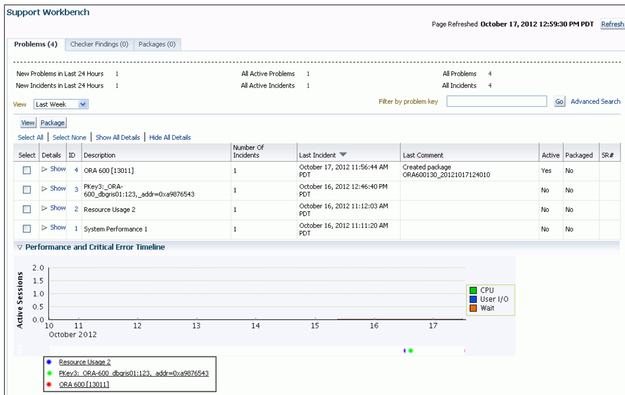
Figure 9-4 Support Workbench Home Page in Cloud Control
