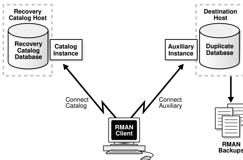
Figure 25-2 Backup-Based Duplication Without a Target Connection
