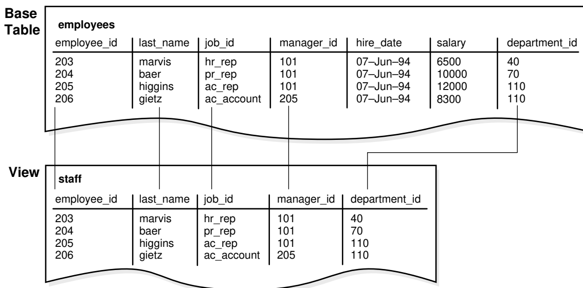
Figure 4-7 View
