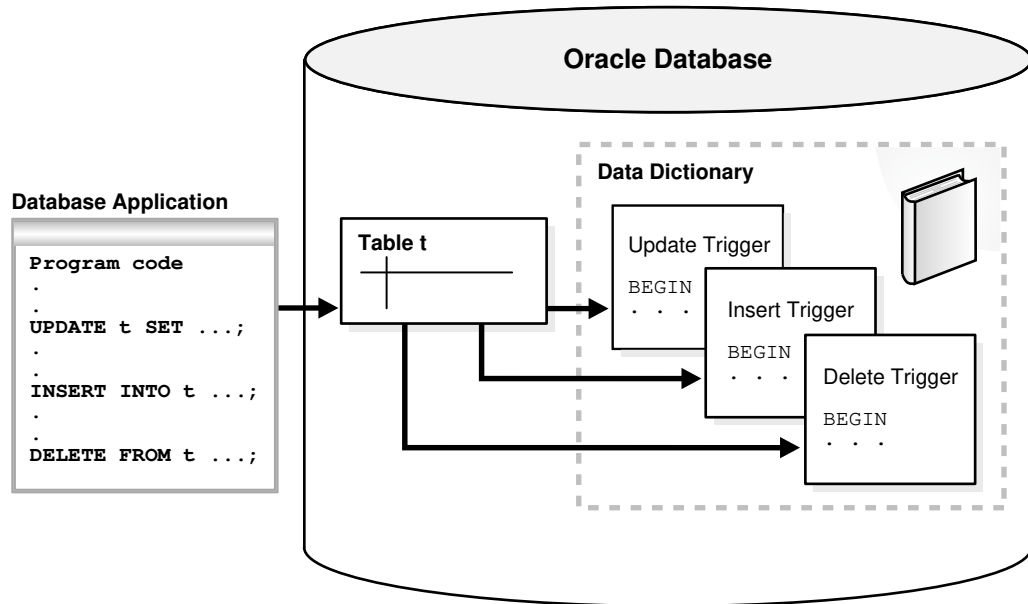
Figure 8-7 Triggers
