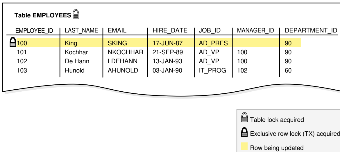
Figure 9-2 Row and Table Locks
