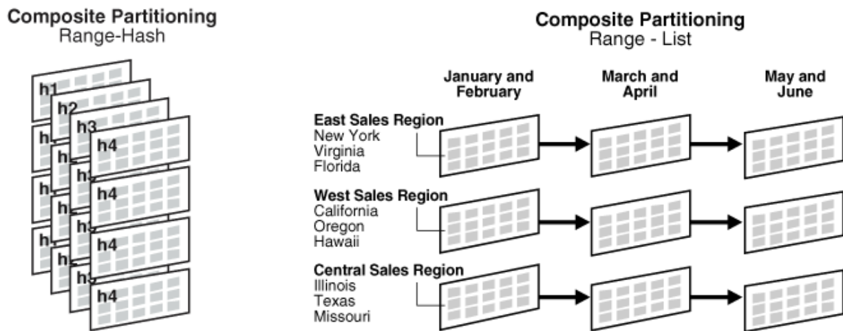
Figure 4-1 Composite Range-List Partitioning
