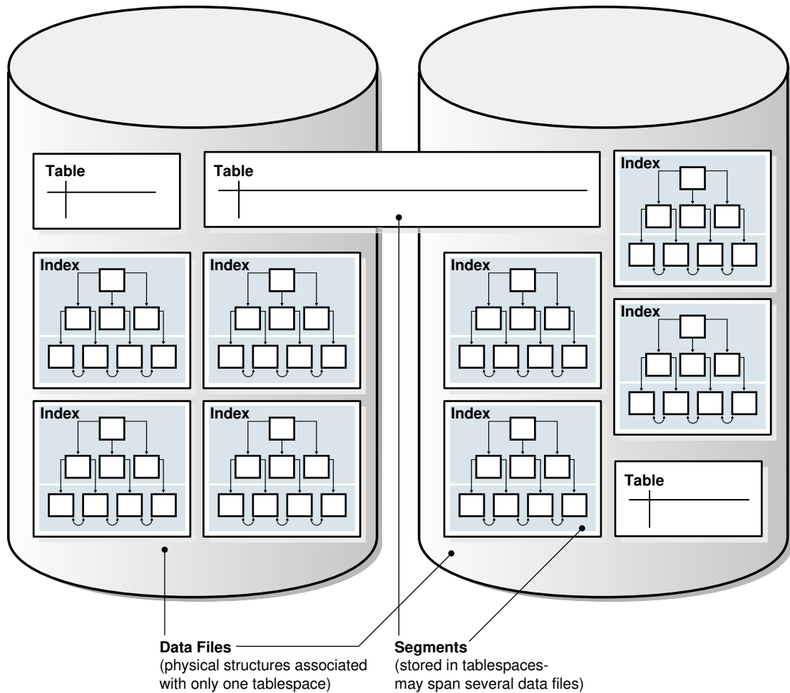
Figure 7-2 Optimizer Components
