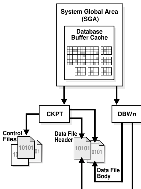
Figure 15-4 Checkpoint Process
