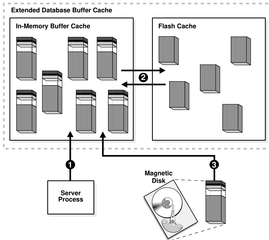
Figure 14-6 Buffer Search
