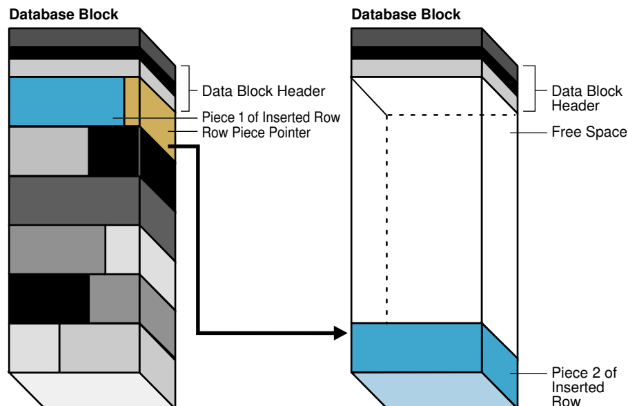
Figure 12-13 Row Chaining
