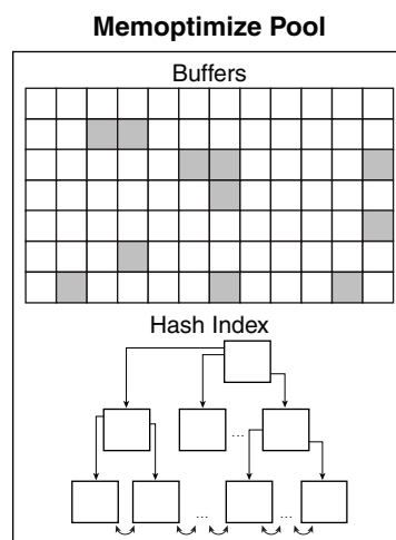
Figure 14-13 Memoptimize Pool
