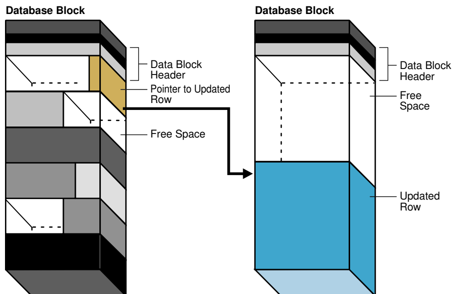
Figure 12-14 Row Migration
