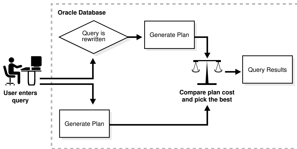
Figure 4-9 Query Rewrite
