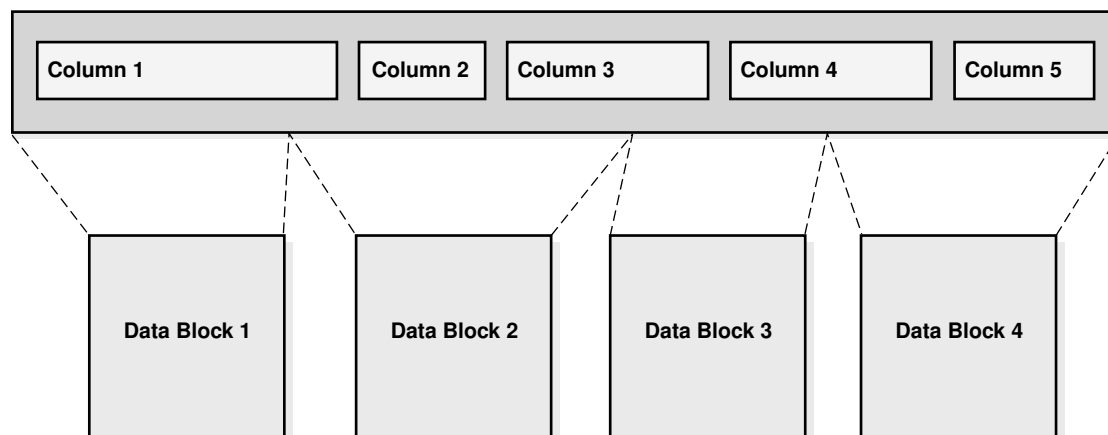
Figure 2-4 Compression Unit
