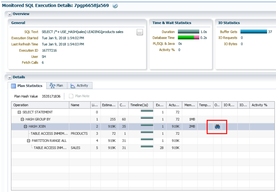
Figure 8-4 Monitored SQL Execution Details Page
