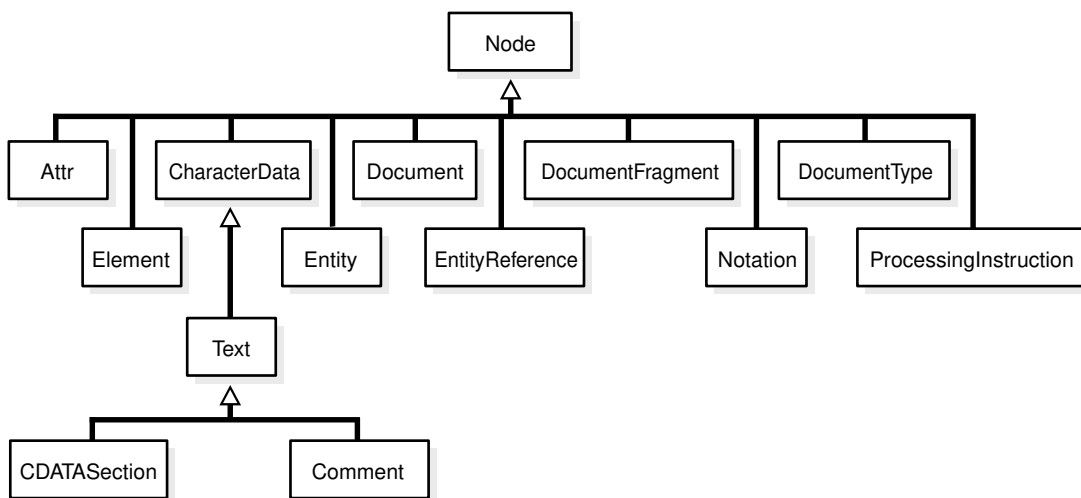
Figure 197-1 Inheritance Diagram for DOM Types
