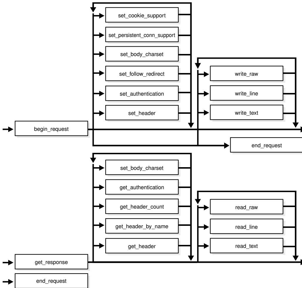
Figure 256-1 Flow of the Core UTL_HTTP Package
