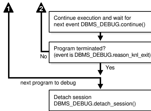
Figure 55-3 Debug Session (Cont.)
