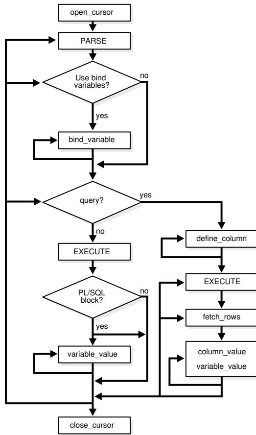
Figure 157-1 DBMS_SQL Execution Flow
