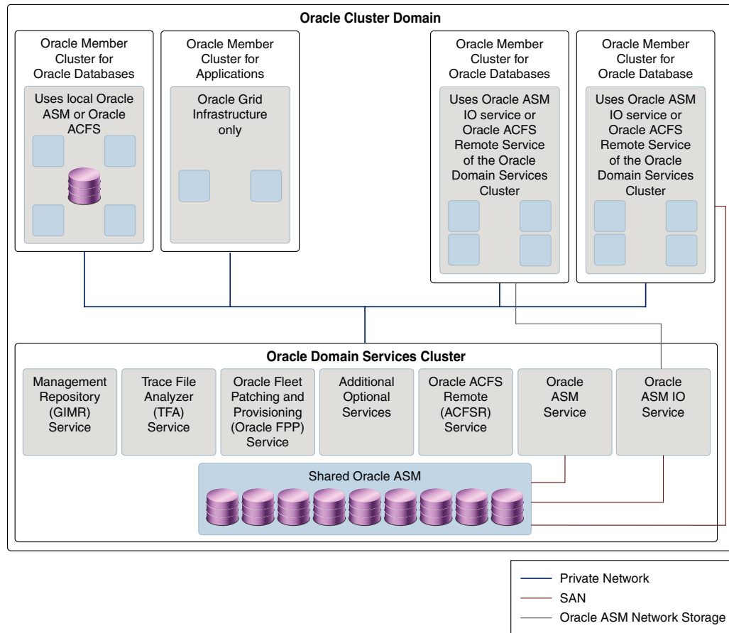
Figure 9-1 Oracle Cluster Domain
