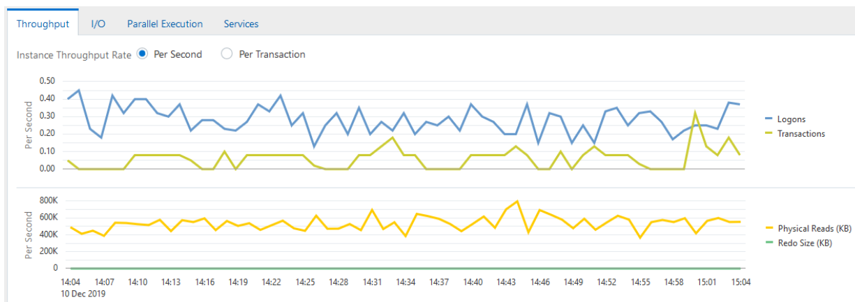
Figure 4-3 Monitoring Throughput
