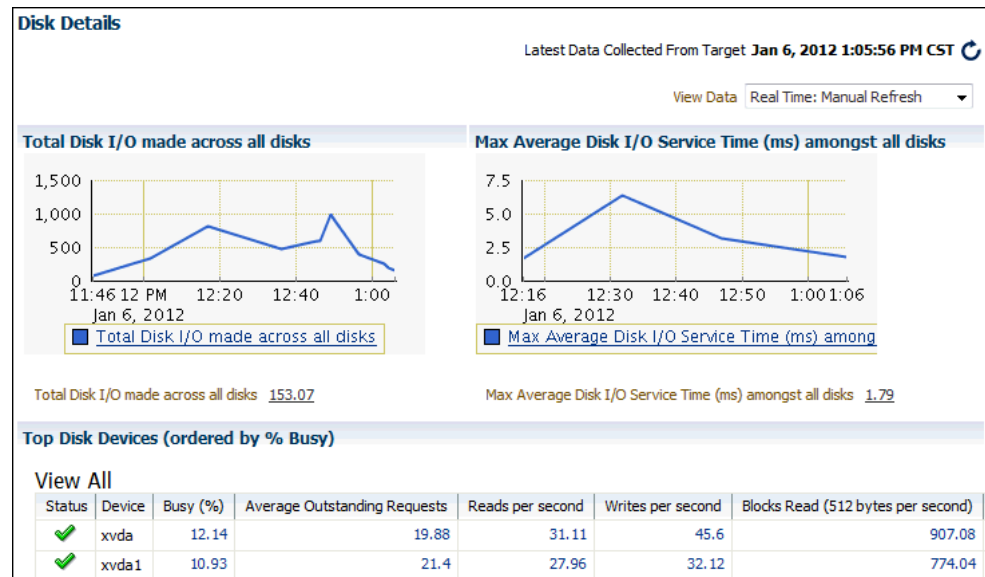
Figure 4-9 Disk Details
