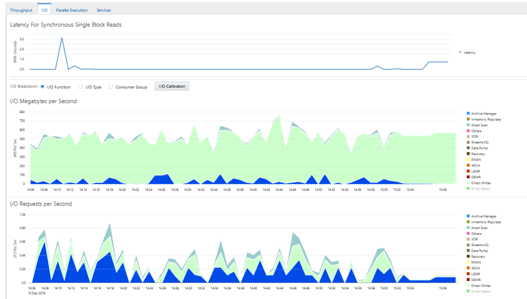
Figure 4-4 Monitoring I/O
