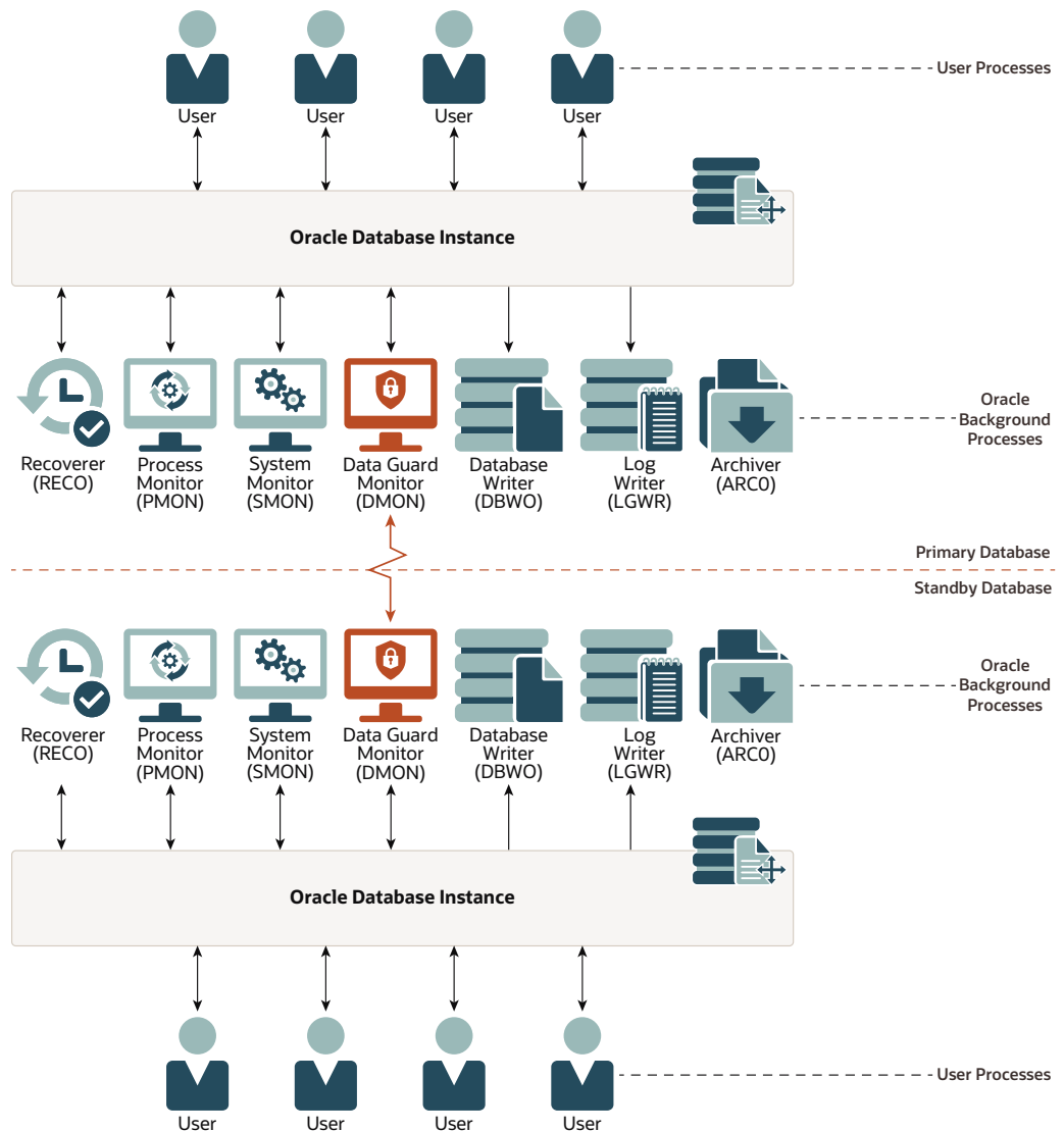
Figure 1-2 Databases With Broker (DMON) Processes
