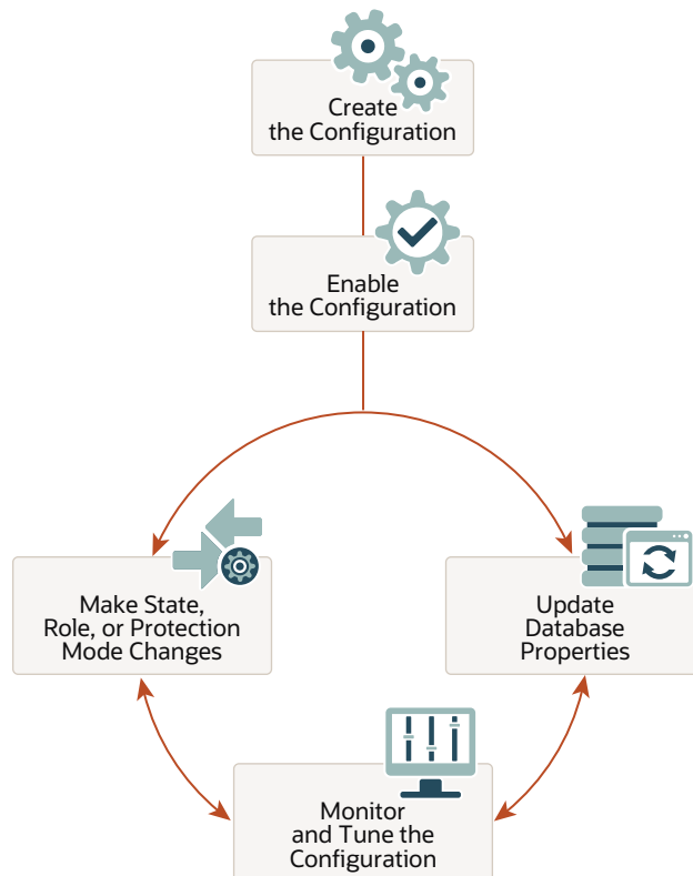
Figure 3-4 Life Cycle of a Broker Configuration and Its Databases
