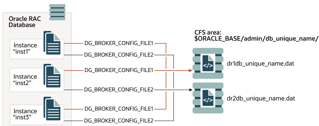
Figure 3-2 Broker Configuration Setup in a CFS Area
