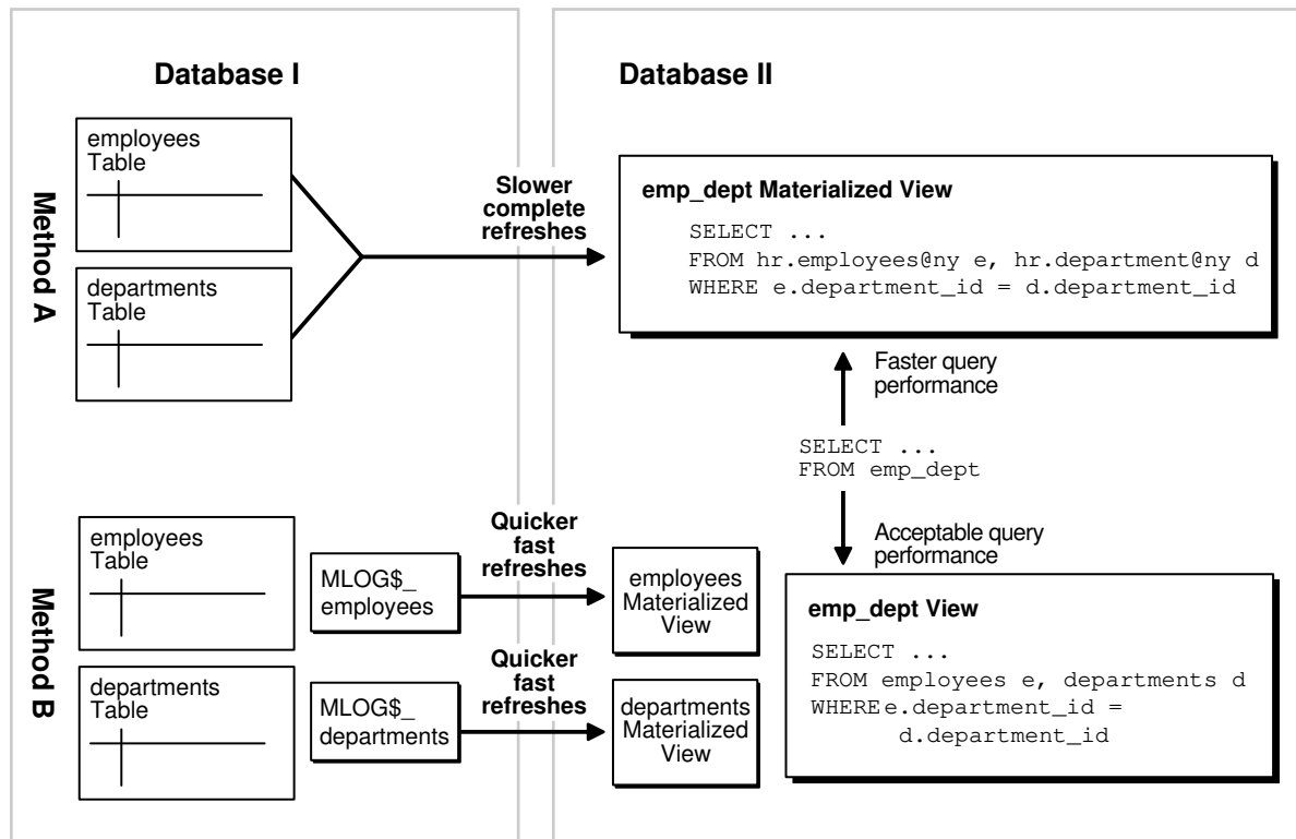
Figure 35-2 Comparison of Simple and Complex Materialized Views
