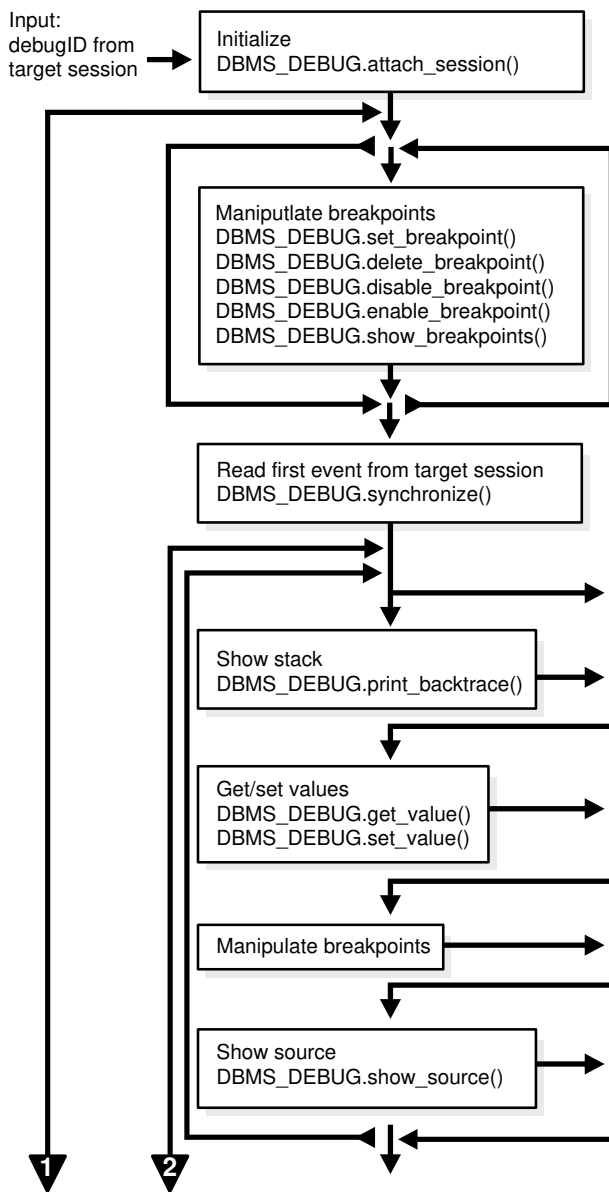
Figure 60-2 Debug Session
