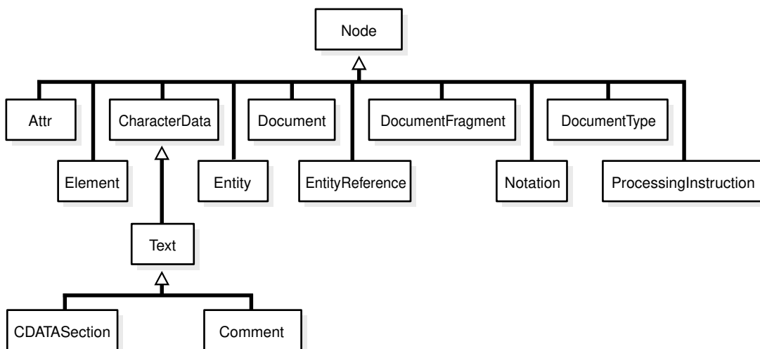
Figure 205-1 Inheritance Diagram for DOM Types
