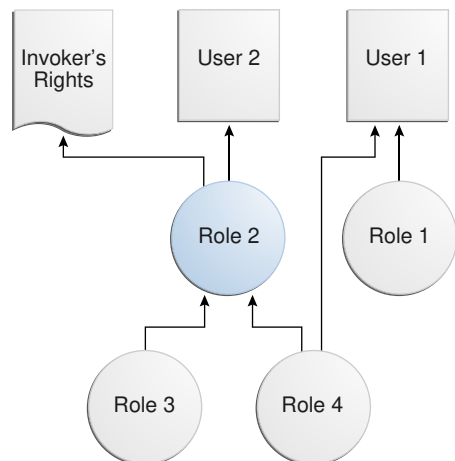
Figure 7-1 Roles Granted to Application Users and Invoker's Right Program Unit
