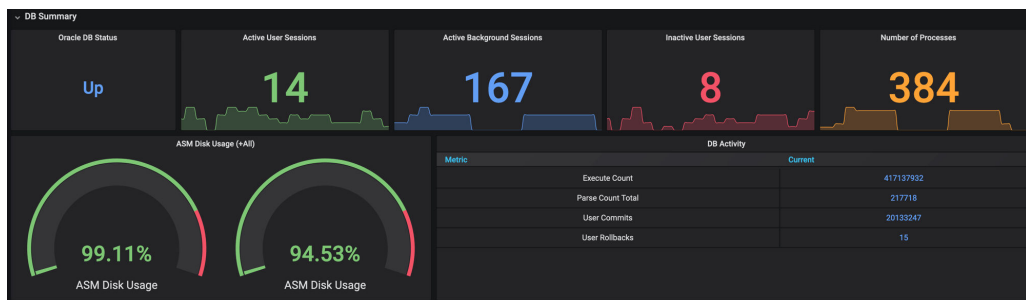
Figure 11-3 Database Summary
