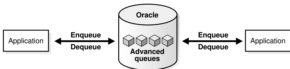
Figure 1-6 Point-to-Point Messaging
