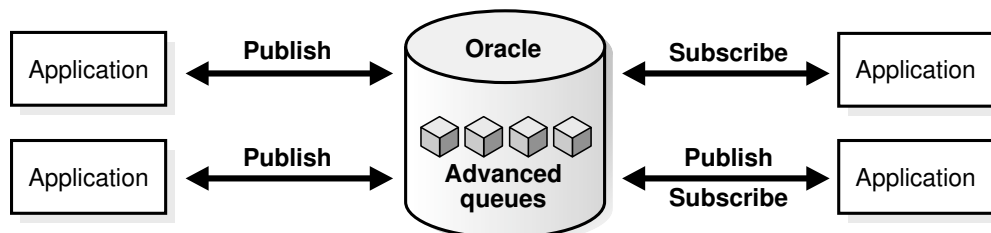
Figure 1-7 Publish/Subscribe Mode
