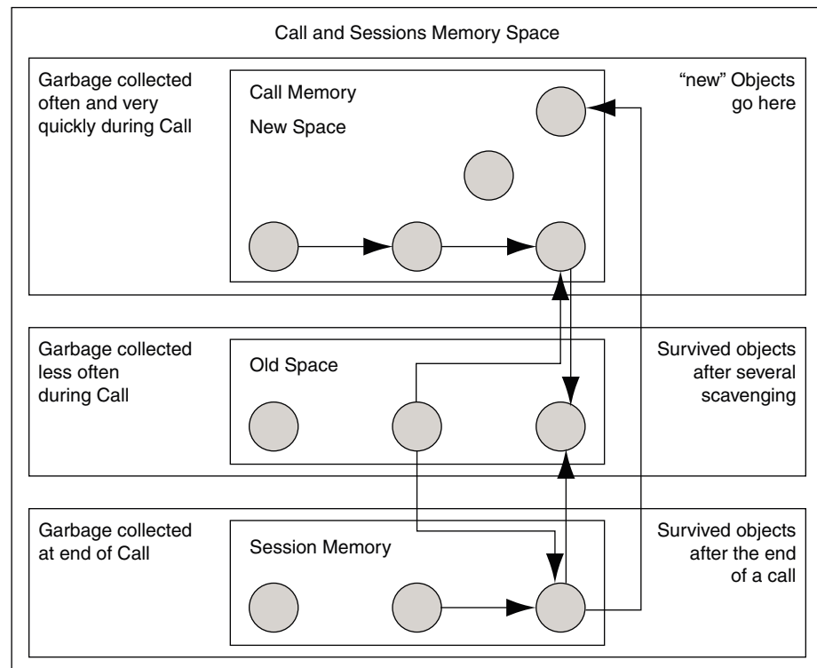
Figure 1-6 Garbage Collection
