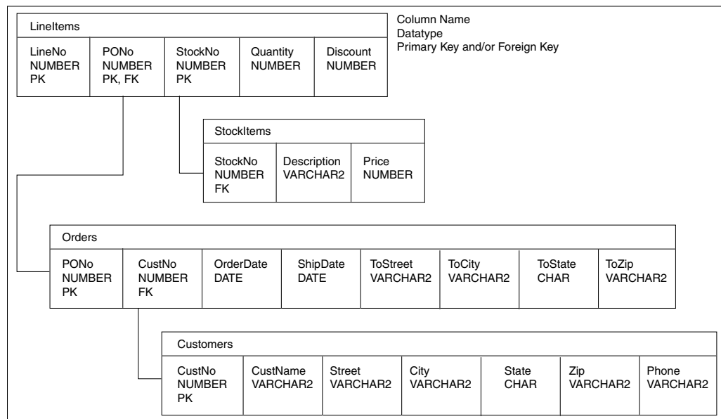
Figure 9-1 Schema Plan for Purchase Order Application
