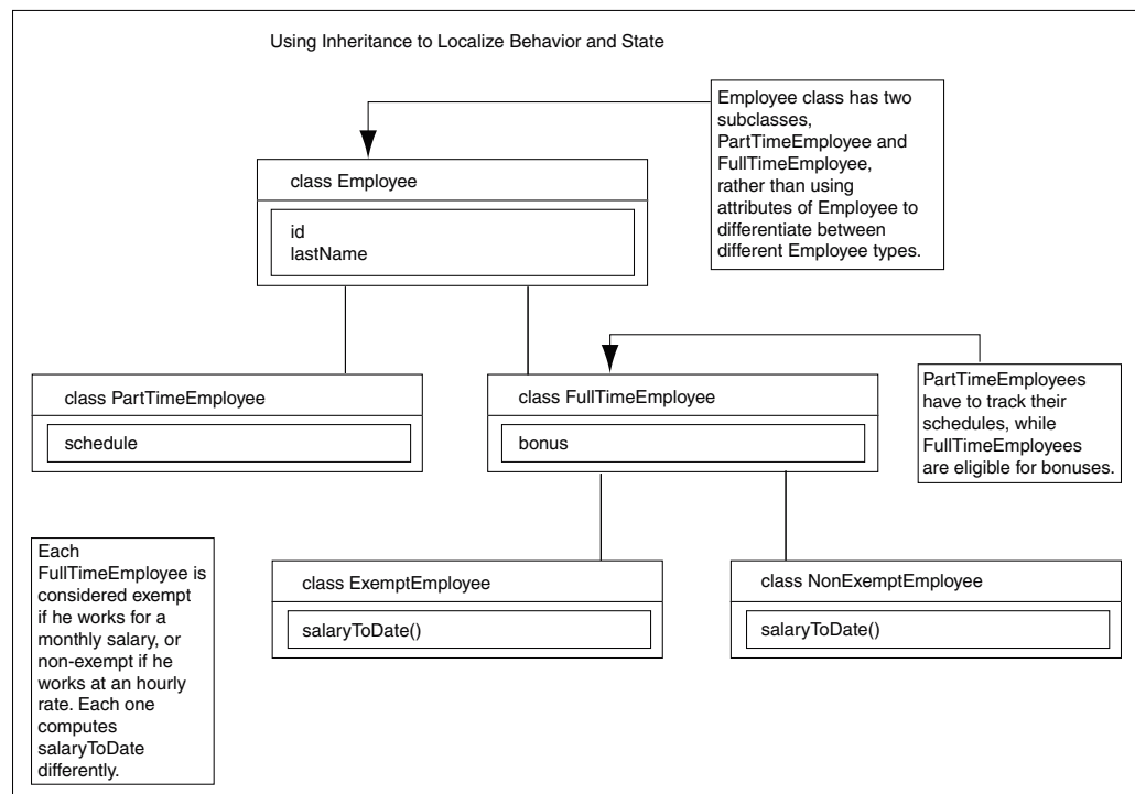
Figure 1-4 Class Hierarchy
